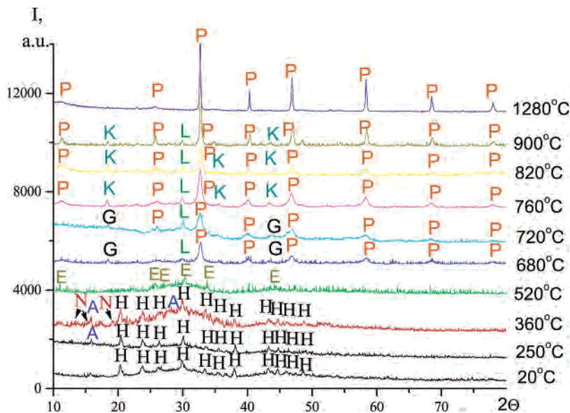
Figure 6. XRPD patterns, obtained at room temperature, of \text{Li}_{0.5}\text{La}_{0.5}\text{TiO}_3 samples prepared by precipitation from solutions after heat treatment at different temperature. A = \text{La}(\text{OH})_3 (36–1421 au); E = \text{La}_2\text{O}_2\text{CO}_3 (37–804 au); G = \text{Li}_2\text{TiO}_3 (33–831 au); H = \text{La}_2\text{O}(\text{CO}_3)_2 \cdot \text{H}_2\text{O} (28–512 au); K = \text{Li}_2\text{Ti}_2\text{O}_5 (38–270 au); L = \text{La}_2\text{Ti}_2\text{O}_7 (28–517 au); N = \text{La}_2(\text{CO}_3)_3 \cdot \text{H}_2\text{O} (25–1400 au); P = perovskite LLTO.
